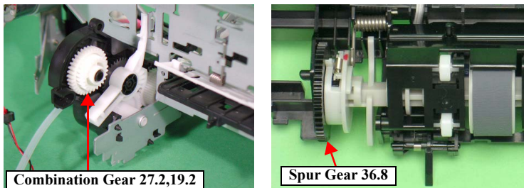
Figure 2-49. Spur Gear 36.8 and Combination Gear 27.2,19.2
