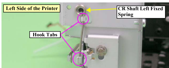
Figure 2-78. Reinstalling the CR Shaft Left Fixed Spring
