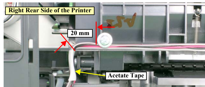
Figure 2-40. Tying the Connector Cables with Acetate Tape
