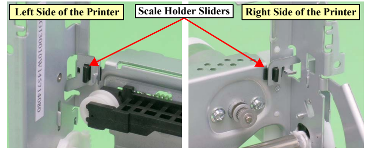
Figure 2-70. Scale Holder Sliders
