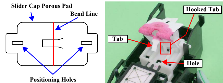
Figure 2-87. Reattaching the Cap Slider Porous Pad
