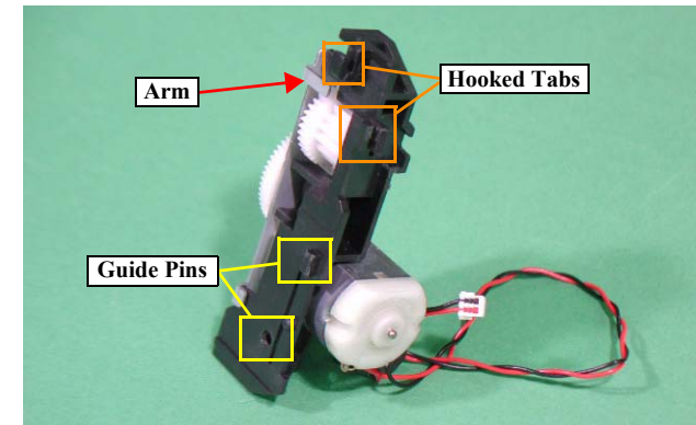
Figure 2-67. Reinstalling the APG Assy.
