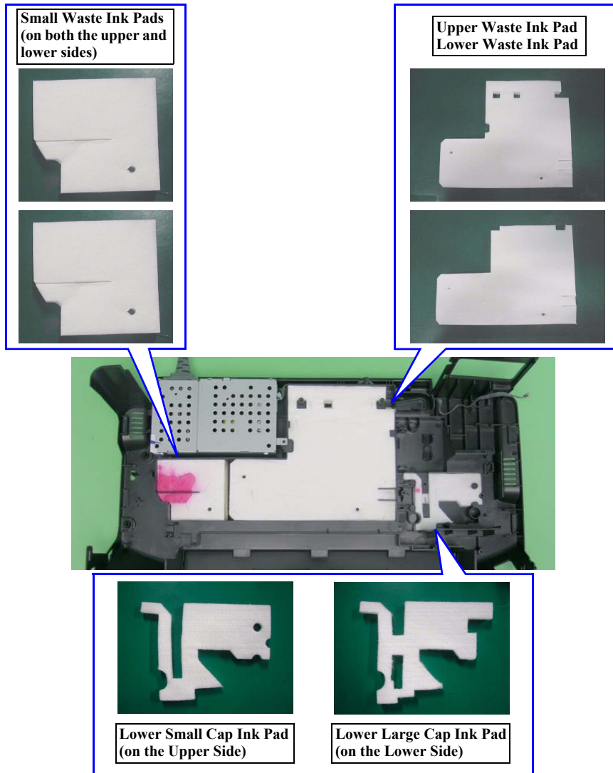
Figure 2-63. Removing the Waste Ink Pads
