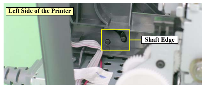
Figure 2-41. Setting and Routing the PF Motor and PG Motor Connector Cables
